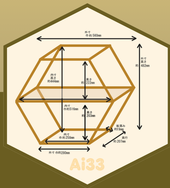
Detail drawing
